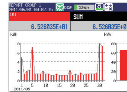
Stacked bar graph You can display and record power consumption of each piece of electronic equipment; useful for energy saving and equipment maintenance as part of environmental protection programs (option).
