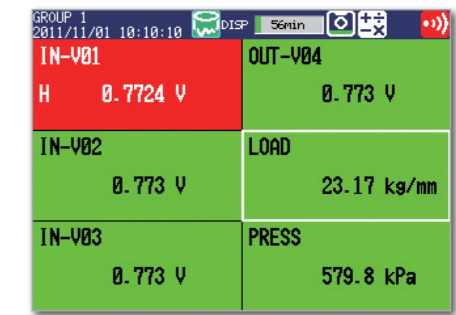
Overview display Displays measurements and alarm statuses on all channels.
